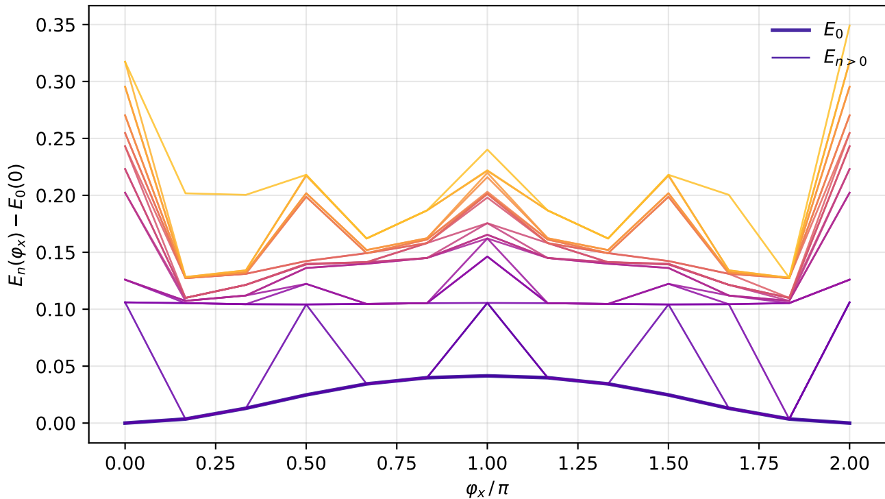
Twist-induced photon dispersion: E_n(\varphi_x) at \varphi_y = \varphi_z = 0 (16-site pyrochlore, J_{\pm} = -0.1J_{zz} )
