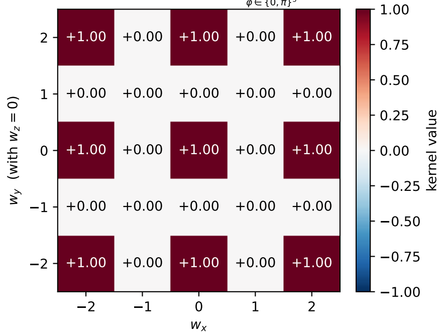
(a) full 8-corner average \frac{1}{8} \sum_{\varphi \in \{0, \pi\}^3} e^{i\mathbf{w} \cdot \varphi}
