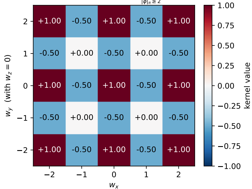
(b) green/olive subset \frac{1}{4} \sum_{|\varphi|_\pi \geq 2} e^{i\mathbf{w} \cdot \varphi}
