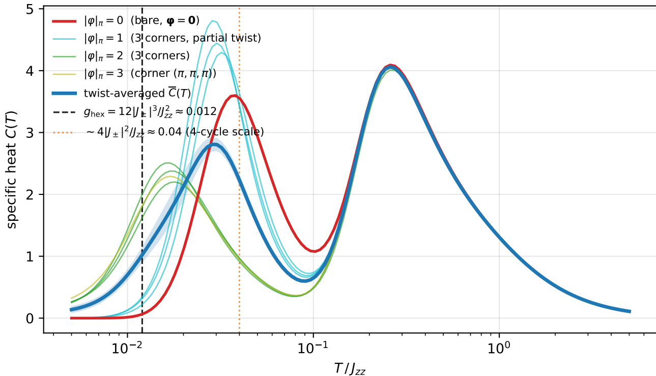
16-site pyrochlore, J_{\pm} = -0.1J_{zz} : C(T) resolved by corner parity class
