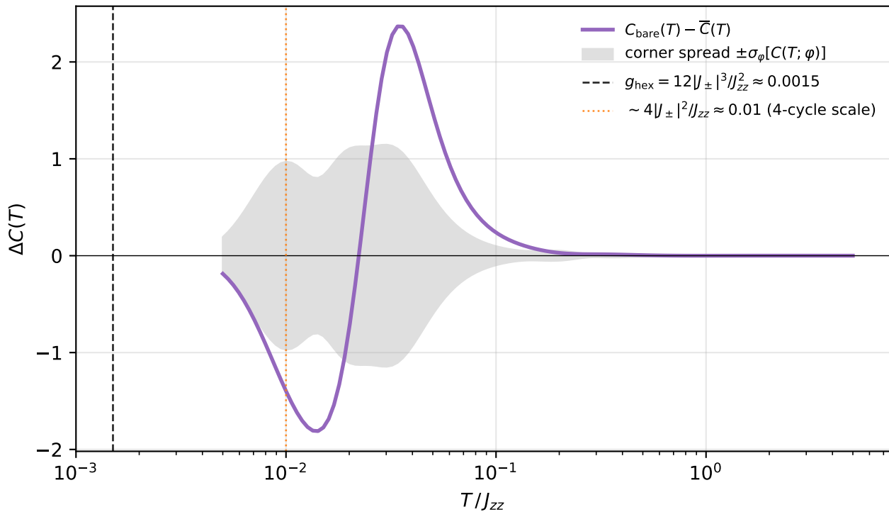
Finite-size correction extracted by twist averaging
