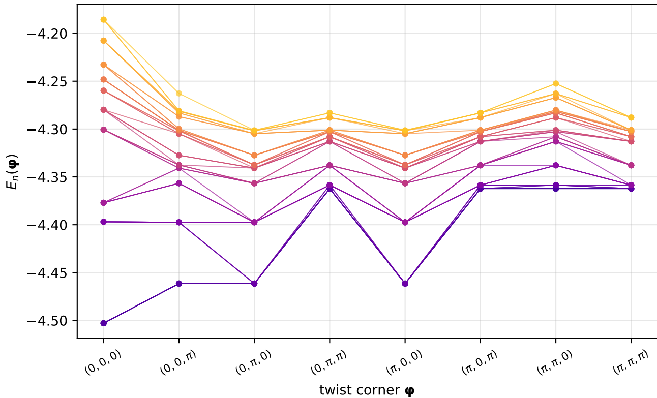
Lowest 48 eigenvalues vs twist corner
