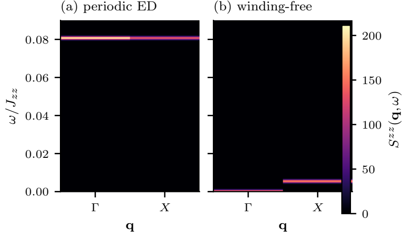
Figure 3: Periodic and winding-free four-sublattice-traced S^{zz}(\mathbf{q}, \omega) on common linear scales. The periodic line begins at 0.08065J_{zz} ; winding-free weight occurs near zero at \Gamma and at 0.005354J_{zz} at each X point.
