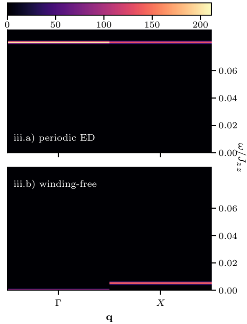
S^{zz}(\mathbf{q}, \omega)
