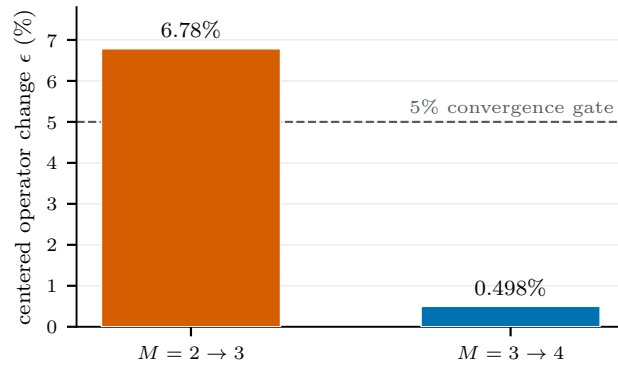
FIG. 1. Successive character-grid convergence of the exact cubic-16 band operator at (J_\pm, J_{\pm\pm})/J_{zz} = (0.046, 0) . Bars show the centered relative Frobenius change in Eq. (30); the dashed line is the preassigned 5% gate.
