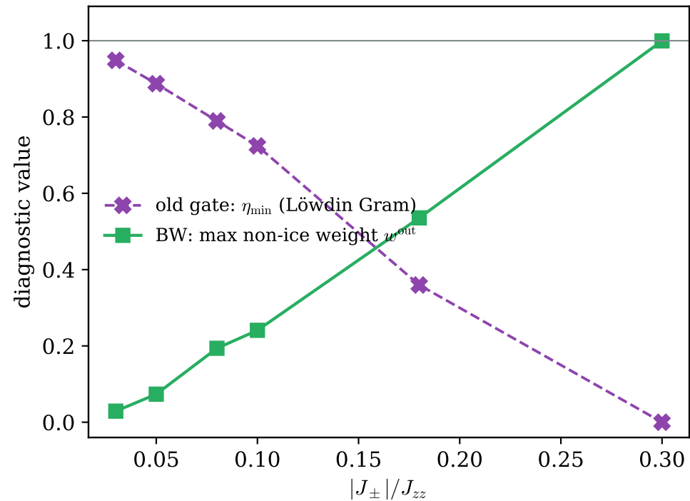
Dressing: smooth where the old gate collapses
