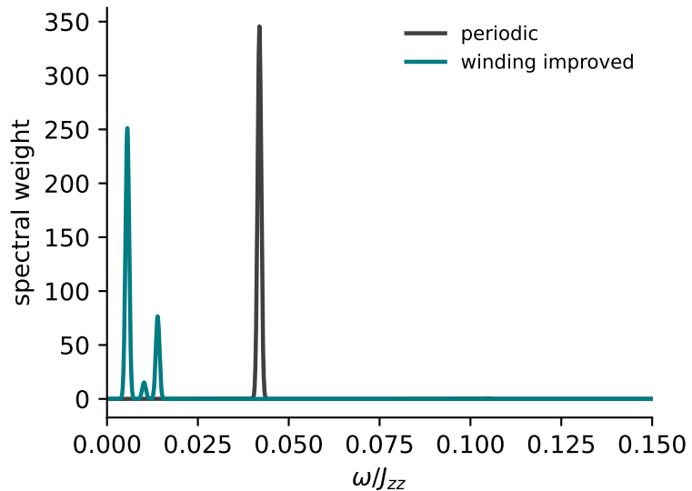
S^{zz}((002), \omega) , cubic average
