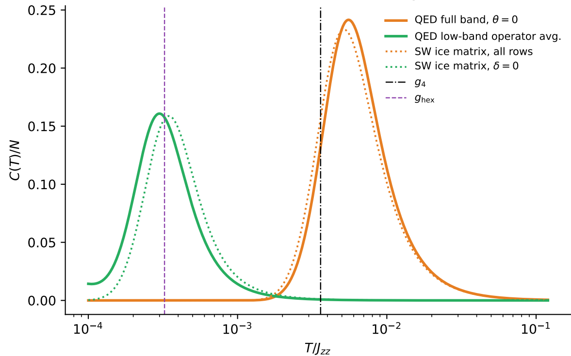
16-site QED low-band character average, J_{\pm} = -0.03
