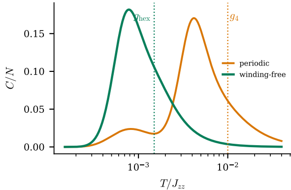
(b) scale correction, J_{\pm}/J_{zz} = -0.05
