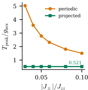
(b) T_{\text{peak}}/g_{\text{hex}}
