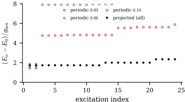
(c) levels in units of g_{\text{hex}}
