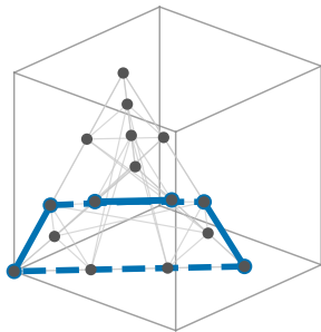
(c) contractible hexagon \mathbf{w} = (0, 0, 0)
