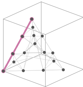
(b) winding four-loop \mathbf{w} = (0, -1, -1)
