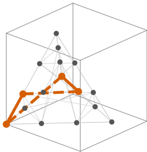
(a) winding four-loop \mathbf{w} = (0, 0, -1)
