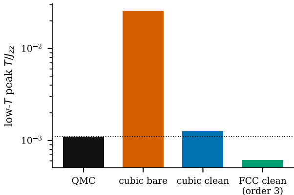
Finite-size and projection hierarchy
