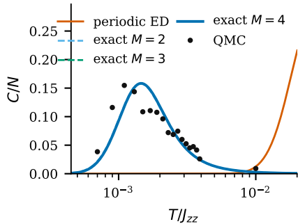
(a) nonperturbative C/N
