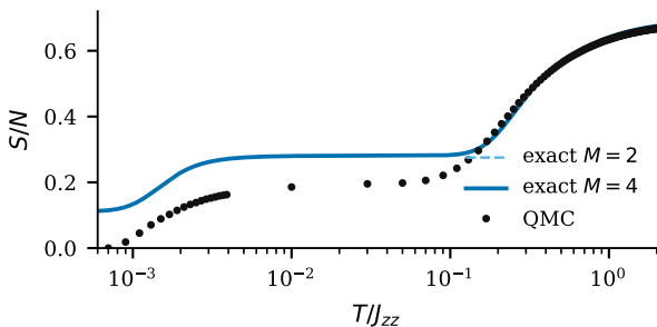
(b) entropy
