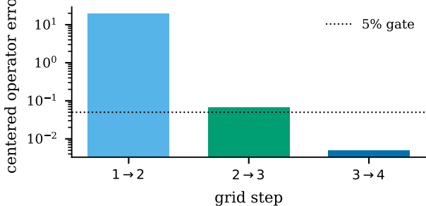
(c) character convergence
