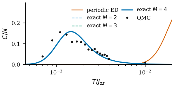
(a) nonperturbative heat capacity
