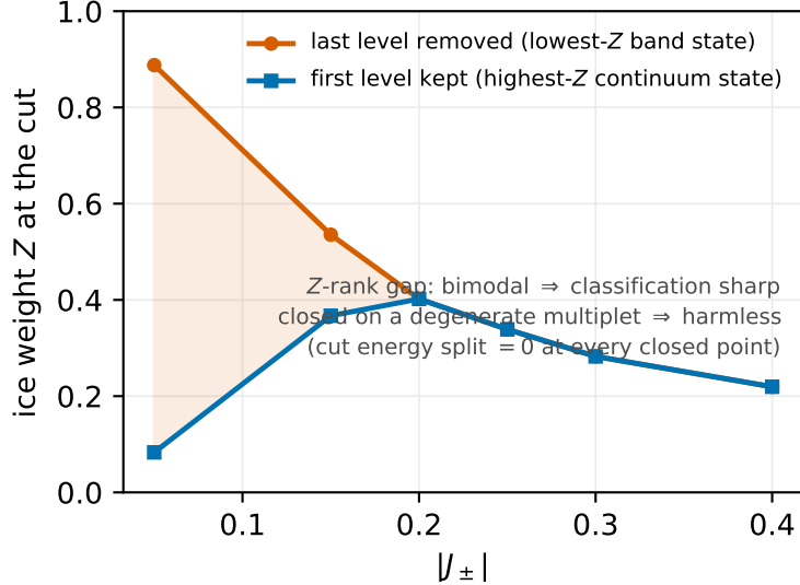
(d) how sharp is the band/continuum cut?
