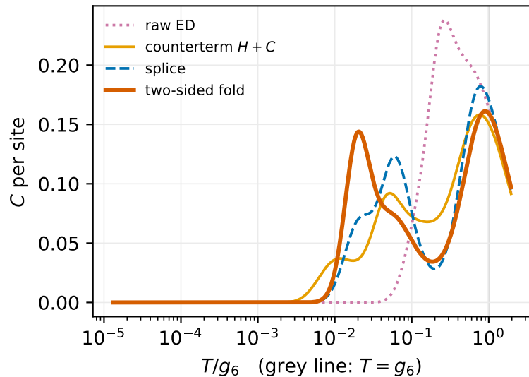
(b) dissolution at J_{\pm} = -0.40
