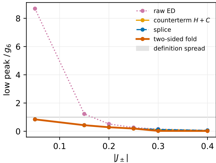
(c) ring-scale peak across definitions
