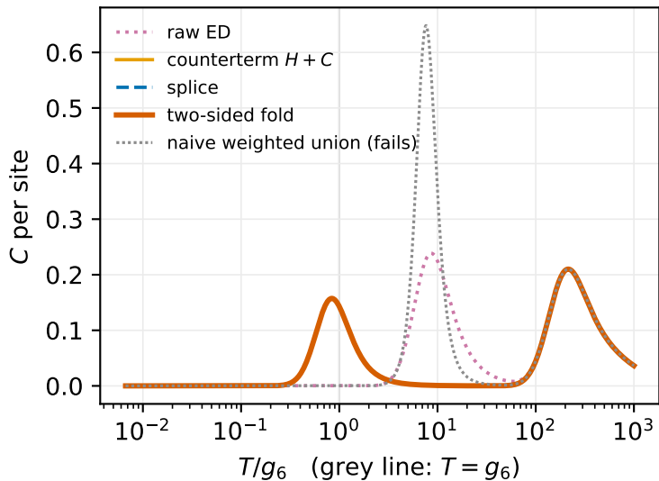
(a) validation at J_{\pm} = -0.05
