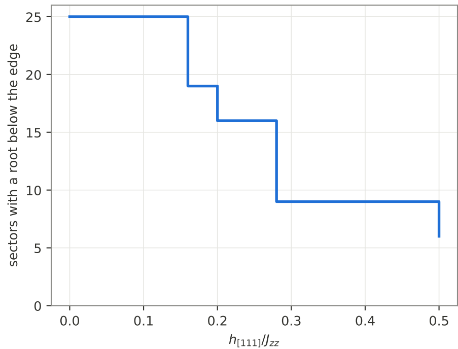
Field-driven sector staircase
