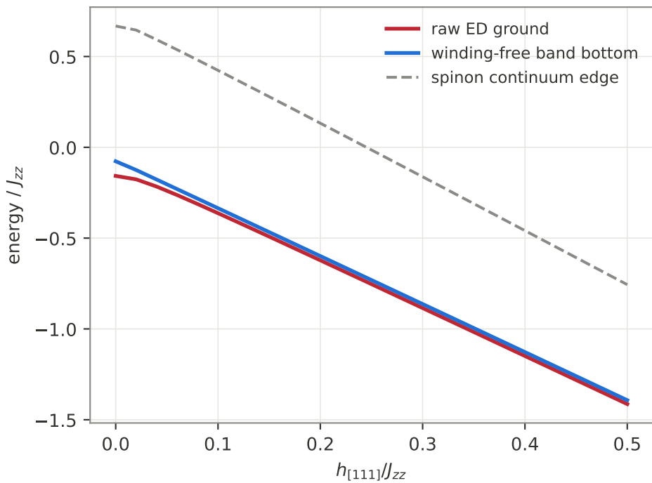
J_{\pm} = -0.05 in a [111] field
