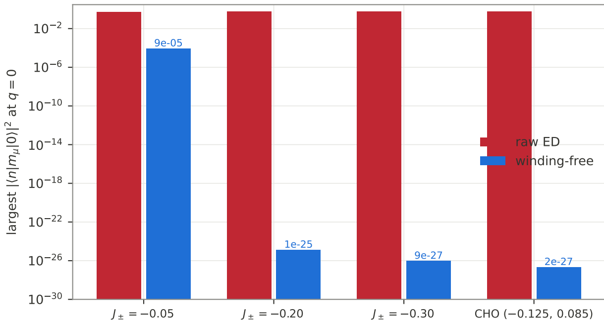
The \Gamma -point longitudinal selection rule
