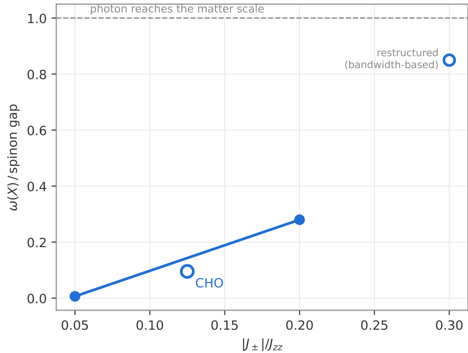
Photon-matter hierarchy of the emergent QED
