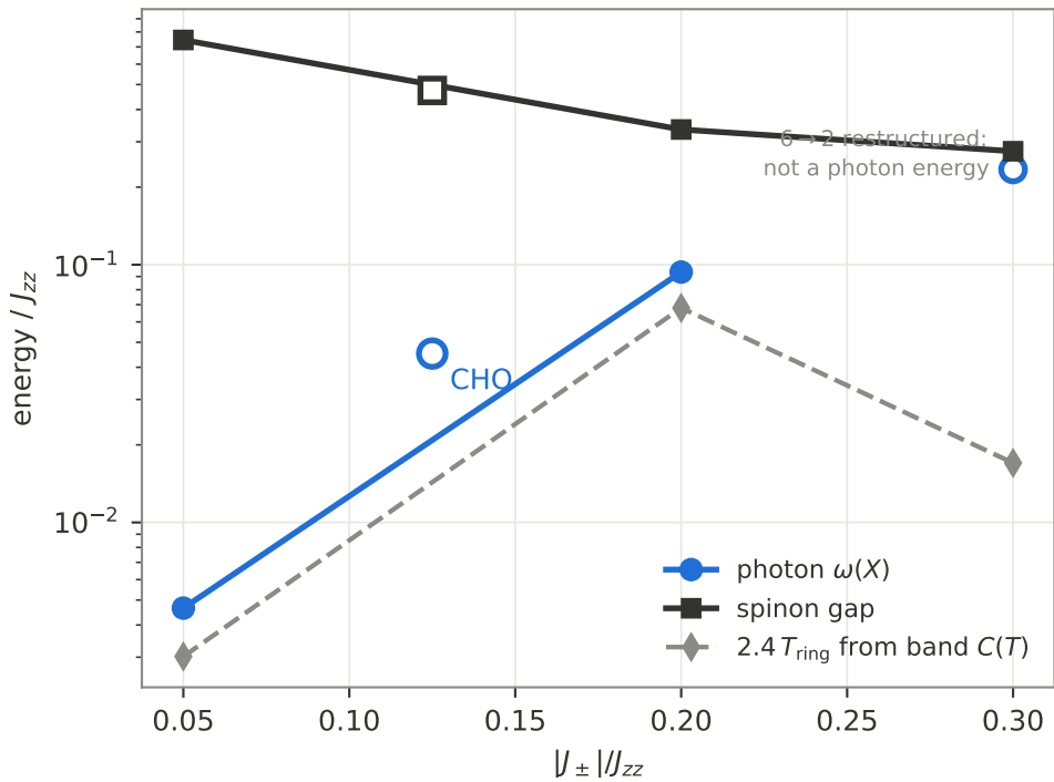
Emergent scales (exact, winding-free)
