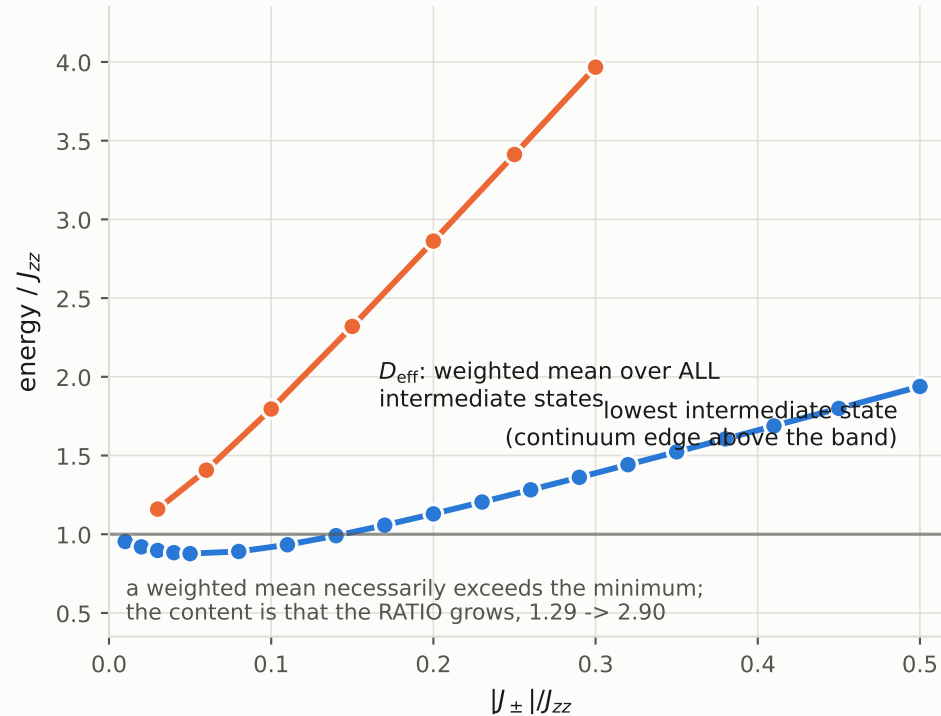
(b) Both scales grow; the denominator outruns the gap
