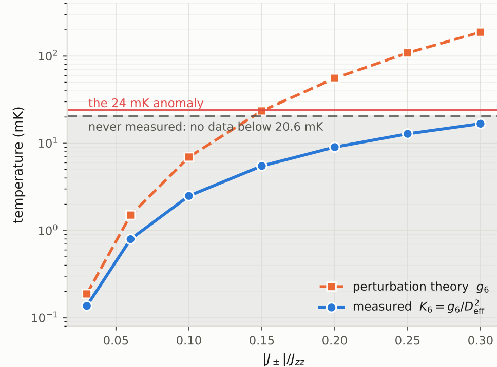
(c) \text{Ce}_2\text{Hf}_2\text{O}_7 : where the photon actually is
