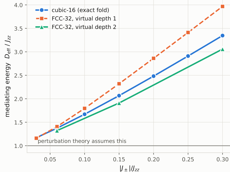
(a) Doubling the crystal barely moves it
