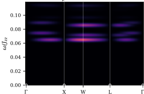
(c) periodic, |\sum_{\mu} A^{\mu}|^2 (U(1)-protected)
