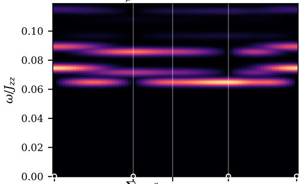
(c) periodic, |\sum_{\mu} A^{\mu}|^2 (U(1)-protected)
