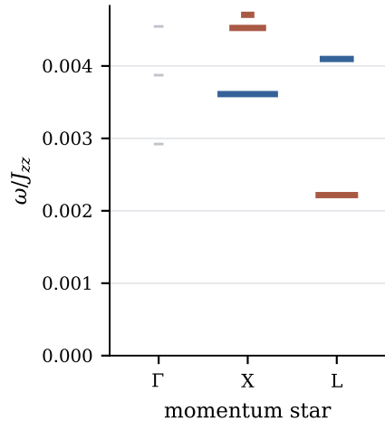
(a) J_{\pm}/J_{zz} = +0.046
