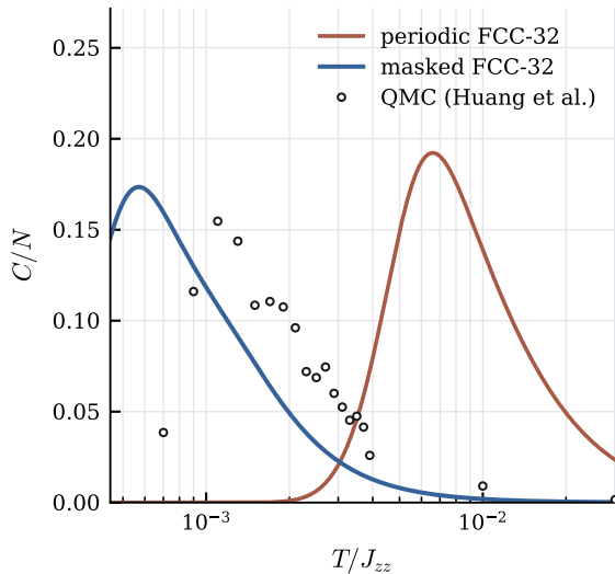
(a) sign-free benchmark, J_{\pm}/J_{zz} = +0.046
