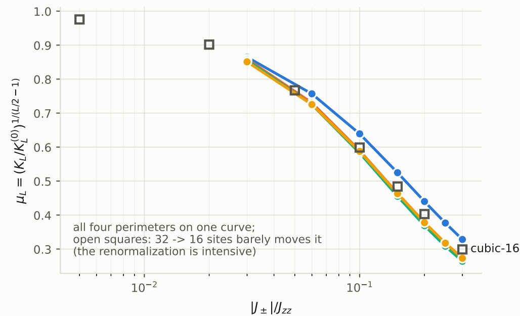
(e) One parameter collapses every perimeter
