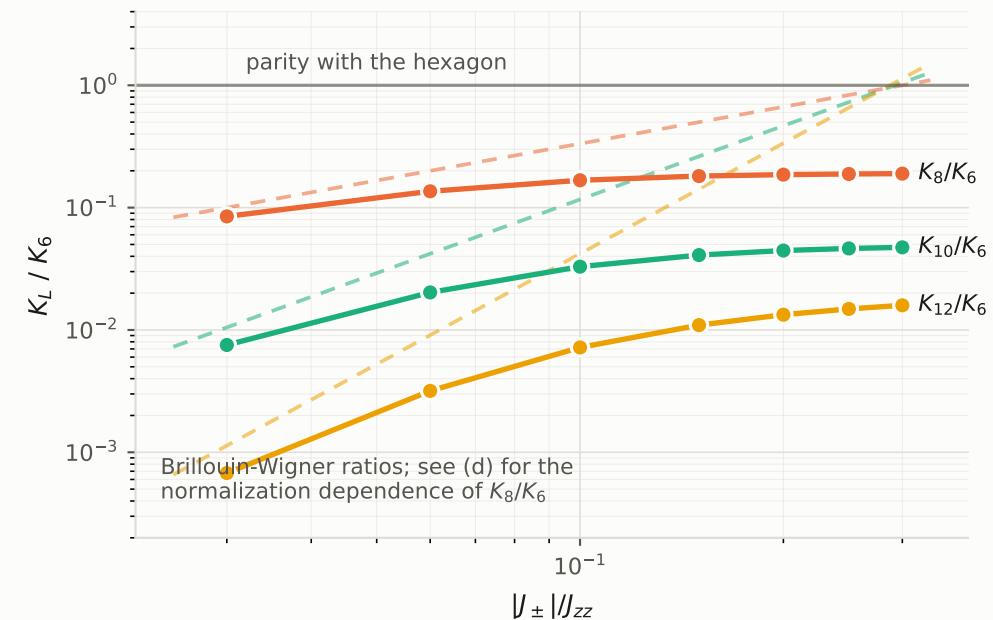
(f) Residual: the hexagon is protected
