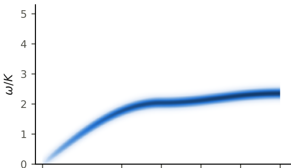
(a) Gaussian theory: S^{zz}(\mathbf{q}, \omega)
