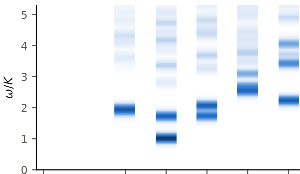
(b) exact compact theory: S^{zz}(\mathbf{q}, \omega)
