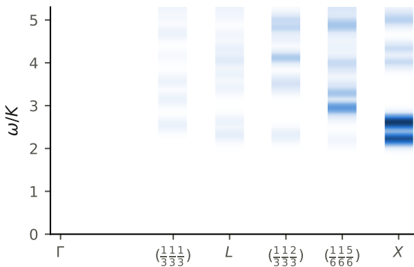
(c) exact: Raman/ultrasound channel \Phi(\mathbf{q}, \omega)
