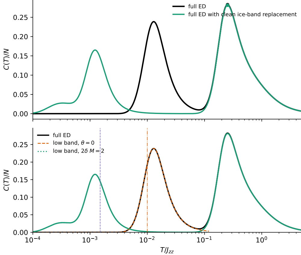
Figure 13: All-temperature full-ED check. The black curve is the exact untwisted microscopic full-ED specific heat for all 65536 states of the 16-site cluster. The green curve keeps every non-ice eigenvalue fixed and replaces only the lowest 90 ice-band eigenvalues by the 2\delta , M = 2 clean twist-projected band, with the band-center shift in Eq. (50). The lower panel zooms into the gauge scale and also shows the two isolated low-band traces. The correction moves only the spurious low-temperature four-loop peak; the larger full-ED peak at T/J_{zz} \simeq 0.253 remains in place.
