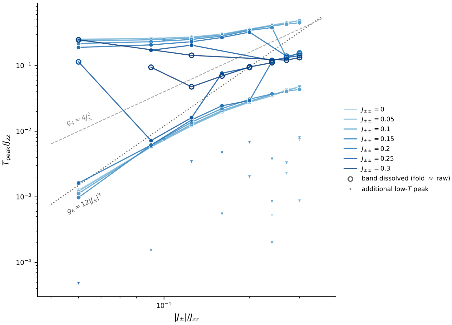
winding-free C(T) peaks across the (J_{\pm}, J_{\pm\pm}) plane (cubic-16 fold)
