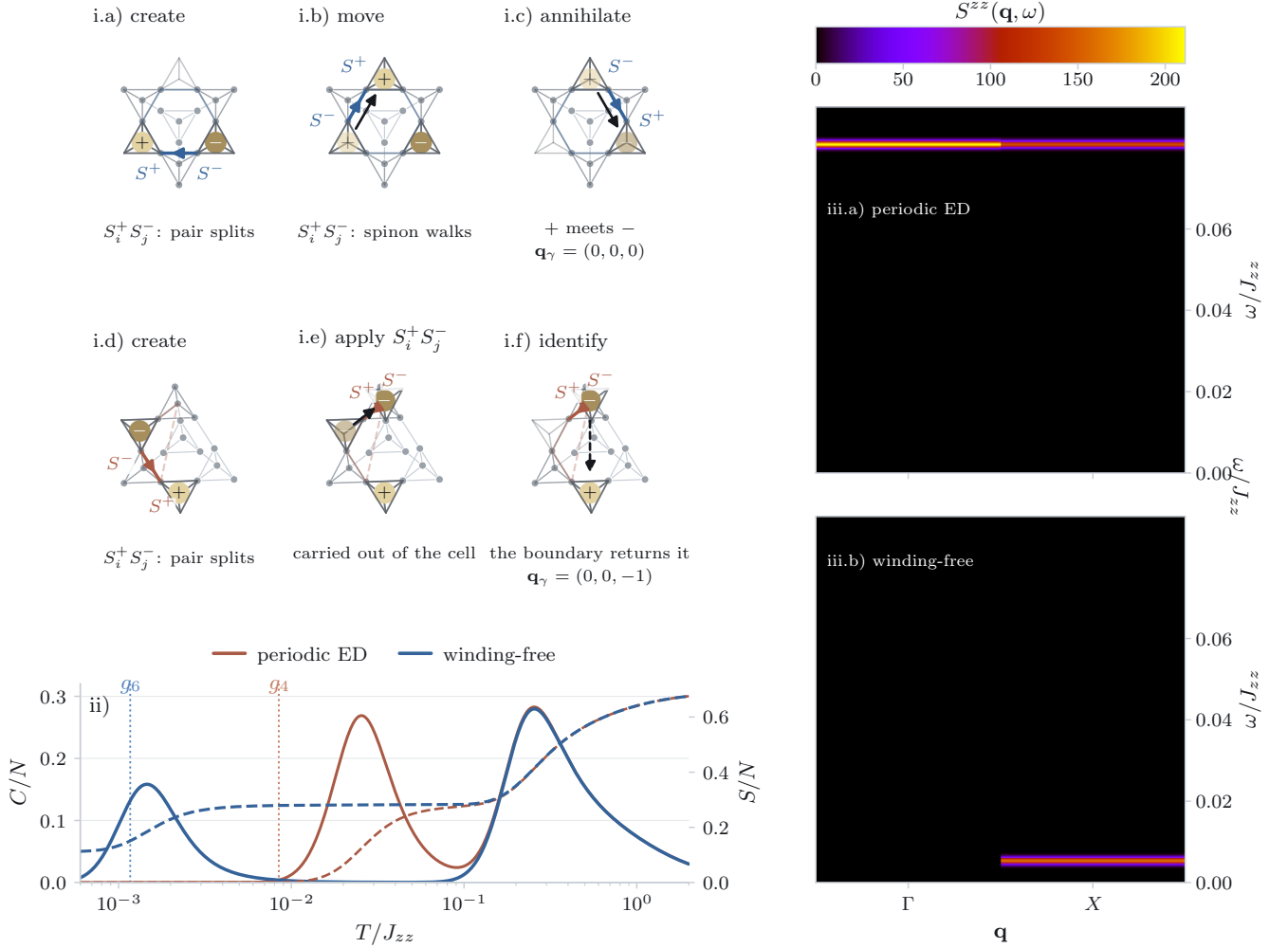
FIG. 1. Microscopic transport and winding removal on cubic-16. (i) A ring exchange stage by stage on the 16-site torus; gray marks the cluster, colored circles the loop, filled versus open symbols the alternating S^z pattern the flip reverses. Each stage highlights the bond its exchange acts on, its endpoints labeled S^\pm by which spin is raised and which lowered. The move leaves the tetrahedron it straddles neutral and charges the two outer ones, so it creates, moves, or annihilates a spinon–antispinon pair. Charges sit at the center of their tetrahedron, whose frame is drawn, light for Q_t > 0 and dark for Q_t < 0 ; an arrow marks every transfer. (i.a)–(i.c) The contractible hexagon: one exchange splits a pair, the next walks the spinon on, the third brings + into - . All inside one cell, and nothing is transported, \mathbf{q}_\gamma = \mathbf{0} . (i.d)–(i.f) The axial four-loop, with its closing step split into the two operations it is actually made of. (i.d) The first exchange splits a pair, exactly as on the hexagon. (i.e) The second exchange then acts, and the antispinon stays put while the spinon is carried out of the cell entirely: the bond it travels along closes only through the periodic boundary, so on the covering lattice the two charges end a full period apart and have not annihilated. (i.f) Only the periodic identification, drawn dashed, maps the spinon back onto its partner and closes the pair. That second operation has no counterpart on the infinite lattice, which is what \mathbf{q}_\gamma = (0, 0, -1) records: the sequence lifts to an open path. The diagonal four-loop behaves identically with \mathbf{q}_\gamma = (1, 1, 0) . The source average of Eq. (10) keeps the hexagon and removes both four-loops. (ii) Heat capacity (solid, left axis) and entropy (dashed, right axis) at (J_\pm, J_{\pm\pm})/J_{zz} = (0.046, 0) , for ordinary periodic ED (orange) and the winding-free replacement of Eq. (11) at M = 4 (blue). Dotted vertical lines mark the perturbative scales g_6 and g_4 of Eqs. (2) and (3); the periodic low-temperature peak tracks the artifact scale g_4 , whereas the projected peak moves down to the ring-exchange scale g_6 . (iii.a),(iii.b) Zero-temperature longitudinal structure factor S^{zz}(\mathbf{k}, \omega) [Eq. (15)] for the periodic band h_{M=4} and the projected band h_{M=4} , on identical linear color scales. Both use the same canonically dressed microscopic S^z probe [Eq. (14)]; results are averaged over the three symmetry-related X points, with broadening \eta = 6 \times 10^{-4} J_{zz} .
