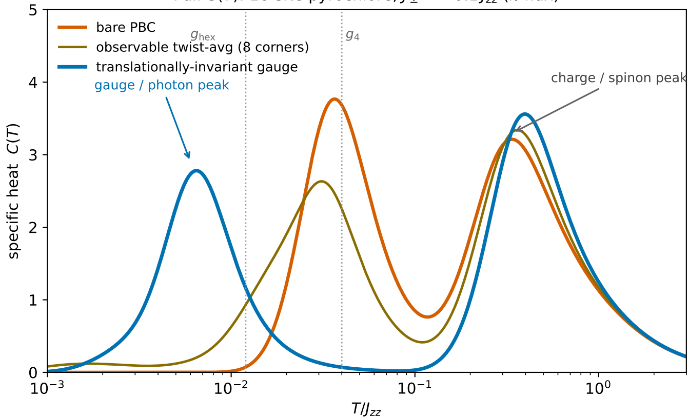
Full C(T) : 16-site pyrochlore, J_{\pm} = -0.1J_{zz} ( \pi -flux)
