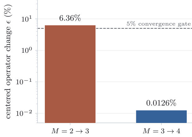
FIG. 1. Successive character-grid convergence of the exact cubic-16 band operator at (J_{\pm}, J_{\pm\pm})/J_{zz} = (0.046, 0) . Bars show the centered relative Frobenius change in Eq. (32) on a logarithmic axis, the two differing by nearly three decades; the dashed line is the preassigned 5% gate.
