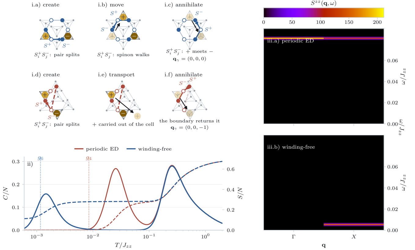
FIG. 1. Microscopic transport and winding removal on cubic-16. (i) A ring exchange stage by stage on the 16-site torus; gray marks the cluster, colored circles the loop, and filled versus open symbols the alternating S^z pattern the flip reverses. Each stage highlights the bond its exchange acts on and labels the endpoints S^+ and S^- by which spin is raised and which lowered. That move leaves the tetrahedron it straddles neutral and charges the two outer ones, so it creates, moves, or annihilates a spinon–antispinon pair. Charges sit at the center of their tetrahedron, whose frame is drawn, light for Q_t > 0 and dark for Q_t < 0 ; the previous stage is faded and an arrow marks every transfer. (i.a)–(i.c) The contractible hexagon: an exchange splits a pair, the next walks the spinon on, and the third brings + into –. Everything happens inside one cell and nothing is transported, \mathbf{q}_\gamma = \mathbf{0} . (i.d)–(i.f) The axial four-loop: the pair splits, the loop then leaves the cell carrying + out through a boundary-crossing bond (dashed), and the pair closes only because the periodic boundary returns that charge to face its partner. Lifted to the covering lattice the sequence is an open path whose ends differ by \mathbf{q}_\gamma = (0, 0, -1) , so + annihilates against an image and not against the – it was born with. The diagonal four-loop behaves identically with \mathbf{q}_\gamma = (1, 1, 0) . The source average of Eq. (10) keeps the hexagon and removes both four-loops. (ii) Heat capacity (solid, left axis) and entropy (dashed, right axis) at (J_\pm, J_{\pm\pm})/J_{zz} = (0.046, 0) , for ordinary periodic ED (orange) and the winding-free replacement of Eq. (11) at M = 4 (blue). Dotted vertical lines mark the perturbative scales g_6 and g_4 of Eqs. (2) and (3); the periodic low-temperature peak tracks the artifact scale g_4 , whereas the projected peak moves down to the ring-exchange scale g_6 . (iii.a),(iii.b) Zero-temperature longitudinal structure factor S^{zz}(\mathbf{k}, \omega) [Eq. (15)] for the periodic band h(\mathbf{0}) and the projected band h_{M=4} , on identical linear color scales. Both use the same canonically dressed microscopic S^z probe [Eq. (14)]; results are averaged over the three symmetry-related X points, with broadening \eta = 6 \times 10^{-4} J_{zz} .
