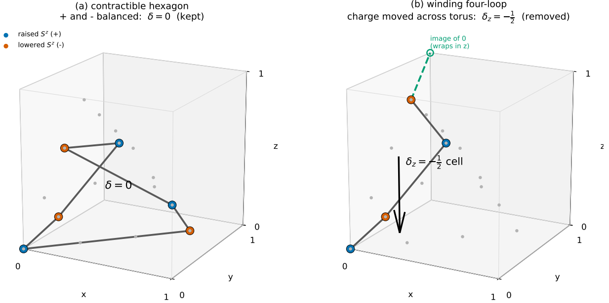
Figure 1: Charge transport on the 16-site cubic pyrochlore cell, \delta = \sum_{\text{raised}} \mathbf{r} - \sum_{\text{lowered}} \mathbf{r} . (a) A contractible hexagon (sites 0, 2, 7, 4, 14, 15) is balanced – the raised (+) and lowered (-) sites share a centroid – so \delta = \mathbf{0} and it is kept. (b) A torus-winding four-loop (0, 2, 7, 5) closes only through the periodic boundary: the dashed bond runs to the periodic image of site 0, wrapping in z . Its raised and lowered charge are offset by half a cell, \delta_z = -\frac{1}{2} , so it is removed. Because the transported charge is half a lattice vector, the flux phase is e^{-i\varphi/2} and must be swept twice (period 4\pi ) to dephase it – the naive 2\pi leaves a residual.
