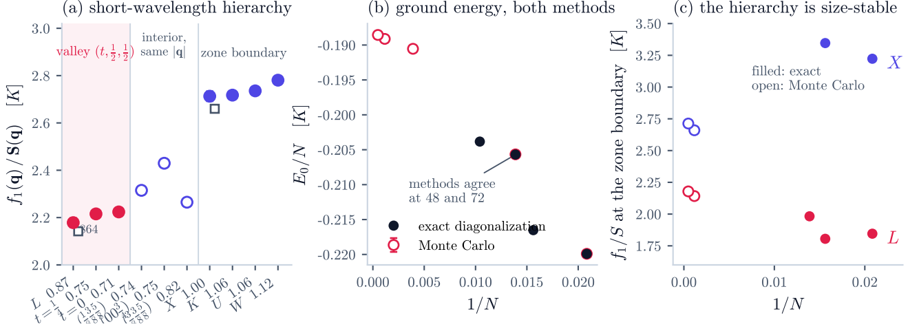
FIG. 4. Large-system ground-state landscape. (a) Feynman ratio f_1(\mathbf{q})/S(\mathbf{q}) on the 2048-site supercell, grouped by geometric role, with |\mathbf{q}| printed under each star. Red: the (t, \frac{1}{2}, \frac{1}{2}) valley, nearly flat along its line. Open circles: interior stars at comparable |\mathbf{q}| — these sit below the boundary plateau only because the branch is still rising with |\mathbf{q}| ; at matched |\mathbf{q}| = 0.75 the valley lies 9–10% (many standard deviations) below the interior star (0, 0, \frac{3}{4}) , which is mid-climb along \Delta , not a second valley. Filled indigo: the true zone-boundary momenta X, K, U, W , 20–25% above L . Open squares: 864-site values at the momenta the two grids share. The complete allowed momentum grid is shown in the Supplemental Material. (b) Ground-state-energy benchmarks comparing exact diagonalization and GFMC. (c) Size evolution of the ratio at L and X across both methods. GFMC constrains the spectral centroid, whereas the finite-cluster diagonalizations establish the dominant low-energy pole.
