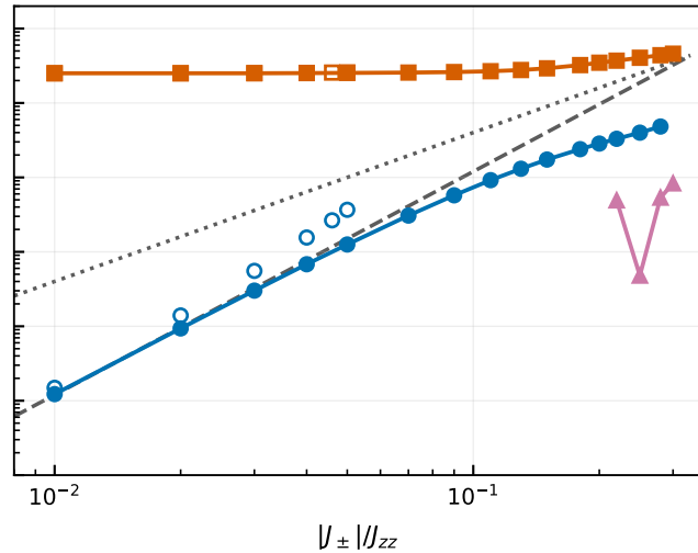
(c) counterterm, anchor solved to 10^{-13}
