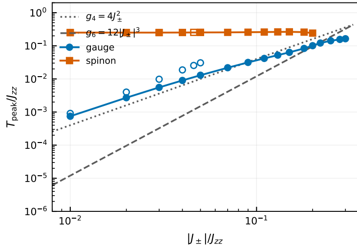
(a) periodic ED (baseline)
