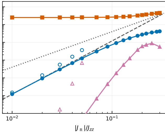
(b) counterterm, anchor iterated 3 ×
