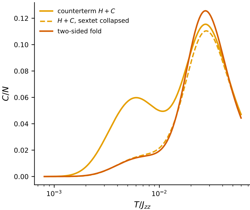
(a) bump 1 is splitting: collapse it, it dies J_{\pm} = -0.20
