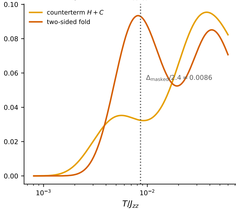
(b) bump 2 sits where the exact gap says J_{\pm} = -0.30, \Delta_{\text{masked}} = 0.0206
