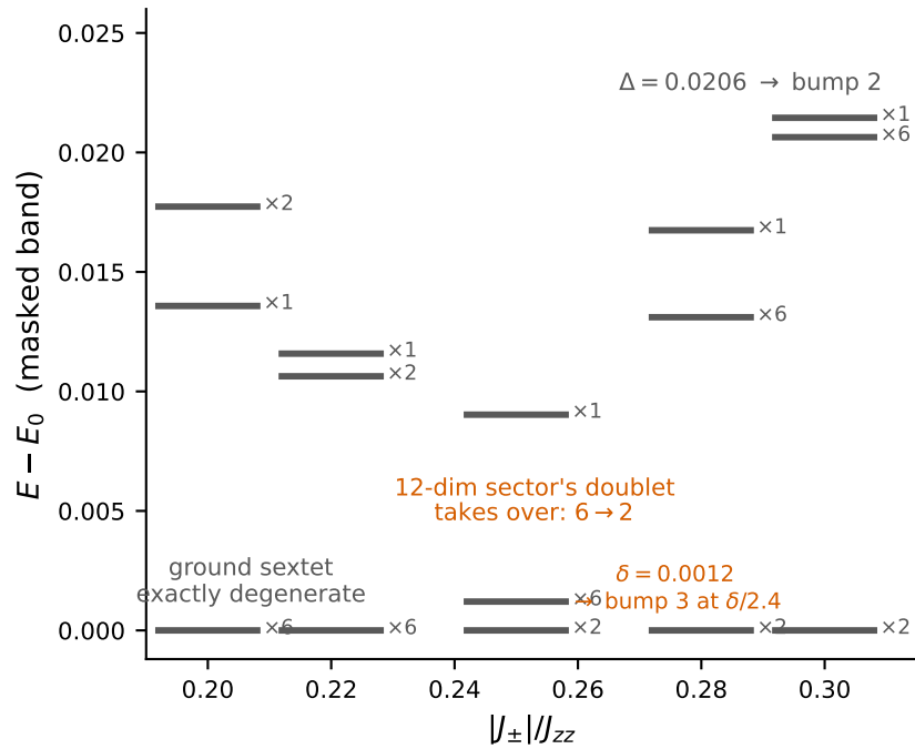
(c) bump 3 is a level crossing lowest exact masked levels
