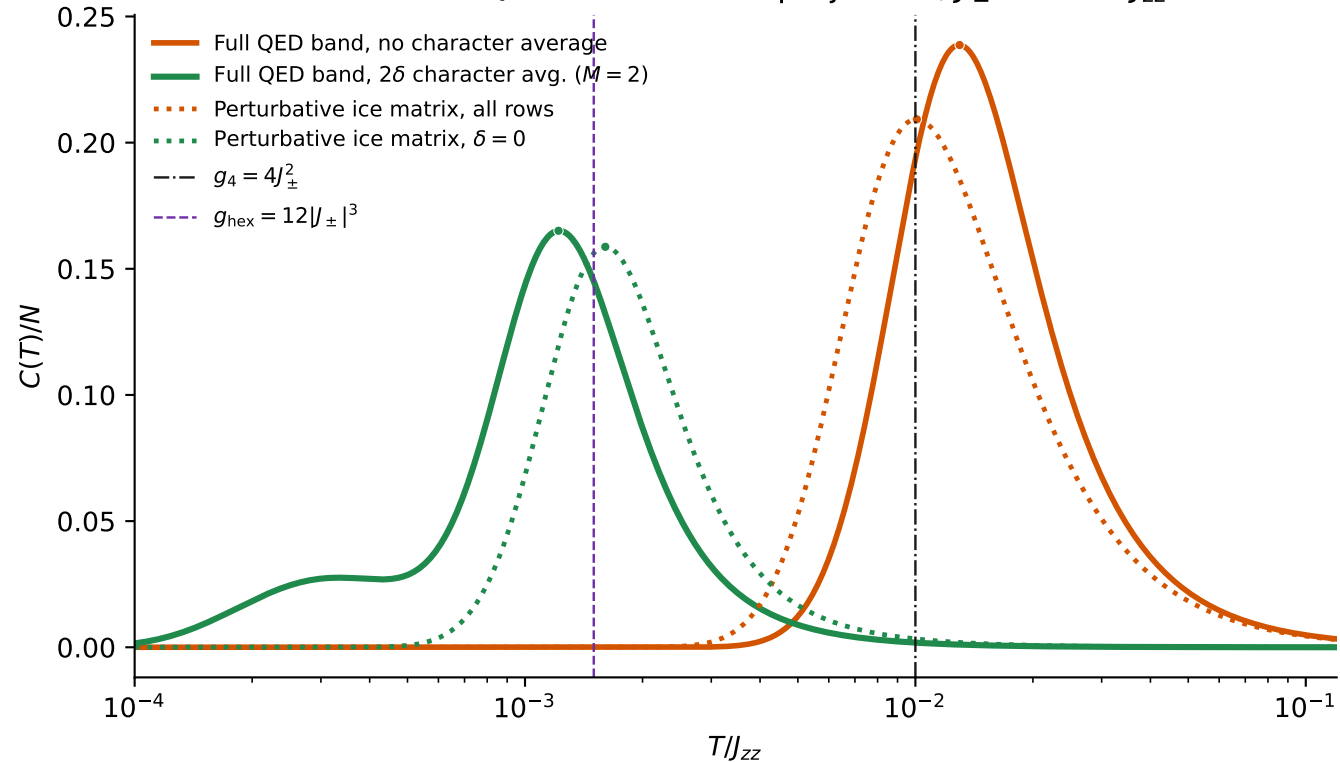
16-site full-QED 2\delta character projection, J_{\pm} = -0.05J_{zz}
