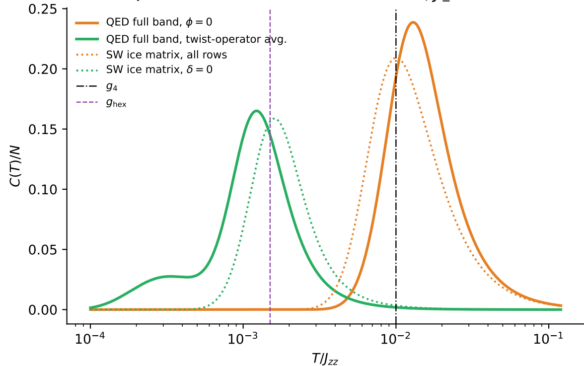
QED full-Hamiltonian twist extraction, J_{\pm} = -0.05
