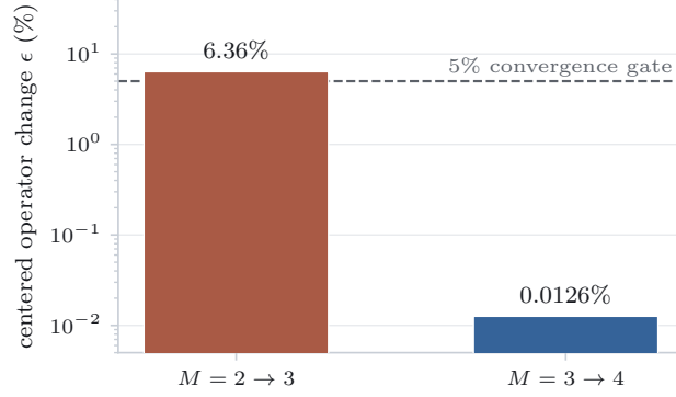
FIG. 1. Successive character-grid convergence of the exact cubic-16 band operator at (J_{\pm}, J_{\pm\pm})/J_{zz} = (0.046, 0) . Bars show the centered relative Frobenius change in Eq. (30) on a logarithmic axis, the two differing by nearly three decades; the dashed line is the preassigned 5% gate.
