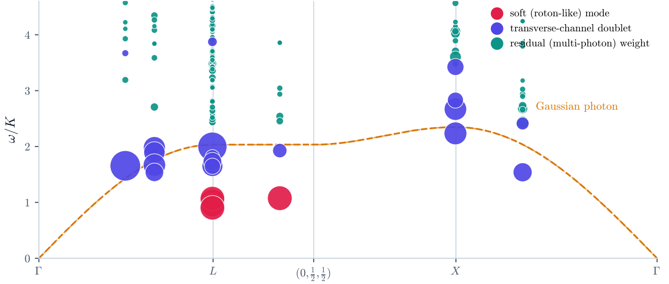
FIG. 2. The S^z spectrum as a dispersion relation. Every exact pole of the diagonalized clusters (48, 64, 72 and 96 spins, overlaid) whose momentum lies on the path \Gamma \rightarrow L \rightarrow (0, \frac{1}{2}, \frac{1}{2}) \rightarrow X \rightarrow \Gamma , placed at its true position; marker area is the level's share of S(\mathbf{q}) at its momentum. Red: the soft roton-like level; indigo: the two dominant transverse-channel levels; teal: the residual (multi-photon) weight. The dashed curve is the Gaussian photon, evaluated analytically on the infinite lattice along the same path with its single fitted scale; the analytic curl reproduces the cluster singular value at L to machine precision. The spectrum tracks the free theory at long wavelength, and at L — and again at the soft-valley momentum (\frac{1}{6}, \frac{1}{2}, \frac{1}{2}) — reconstructs around a pole at roughly half the free-theory energy. The leg (0, \frac{1}{2}, \frac{1}{2}) \rightarrow X contains no cluster momentum and is shown for the free theory only.
