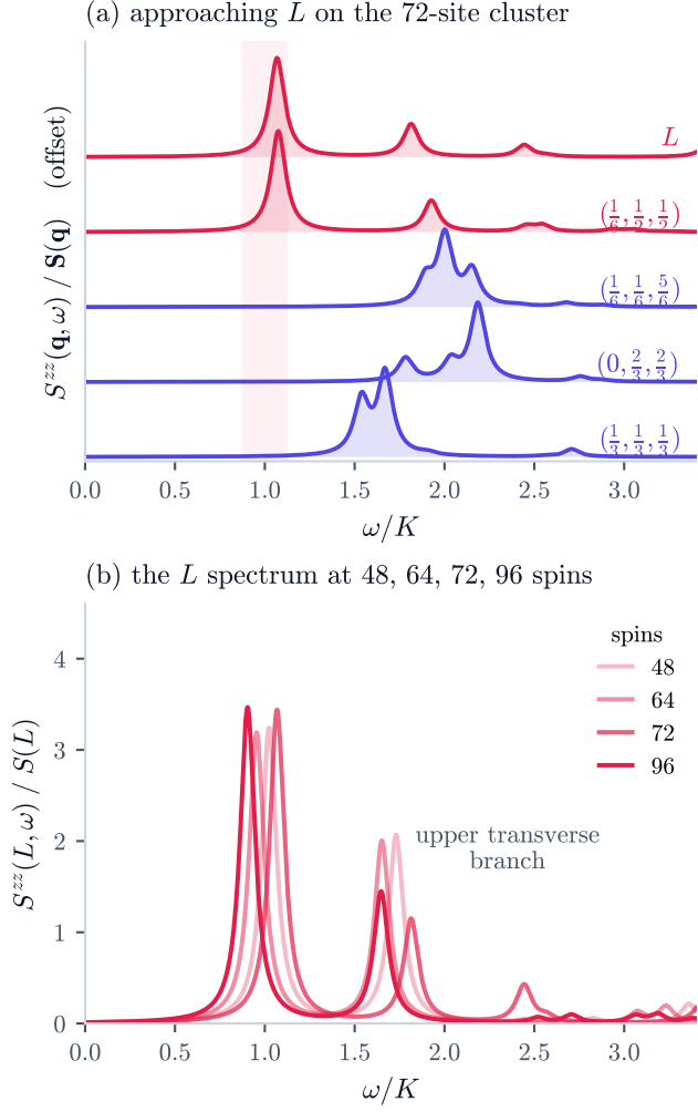
FIG. 5. The mode itself: exact S^{zz}(\mathbf{q}, \omega) near L . (a) The 72-site spectrum at five momenta, each normalized by its own S(\mathbf{q}) ; every pole is exact (Lanczos continued fraction with the sum-rule gate at 1.0000), broadened by a display-only \eta = 0.05K . At the three photon-like momenta the response peaks at 1.5–2.2 K ; at L and at the soft-valley momentum (\frac{1}{6}, \frac{1}{2}, \frac{1}{2}) (Sec. XII A) it collapses onto a single dominant pole near 1 K carrying over half the weight (shaded band). (b) The L -point spectrum at all four diagonalized sizes, overlaid: the soft pole sits at 0.90–1.07 K with about half the weight at every size, the upper transverse branch at 1.65–1.81 K . Nothing here is fitted or extrapolated; the figure is the spectrum.
