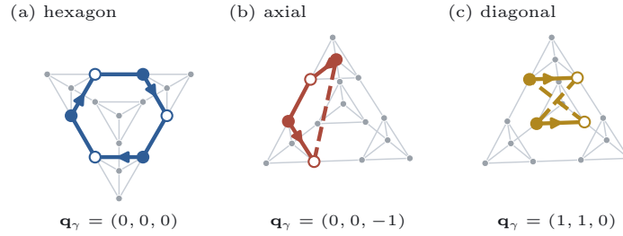
Figure 1: The actual cubic-16 pyrochlore network without an external cubic frame. The two four-loop classes close through periodic bonds (dashed) and carry finite \mathbf{q}_\gamma = 2 \sum_\ell \Delta \mathbf{p}_\ell , shown as the dark resultant of the colored spin-transfer arrows. The contractible ring is viewed normal to its plane, making its D_6 geometry and \mathbf{q}_\gamma = 0 explicit.
