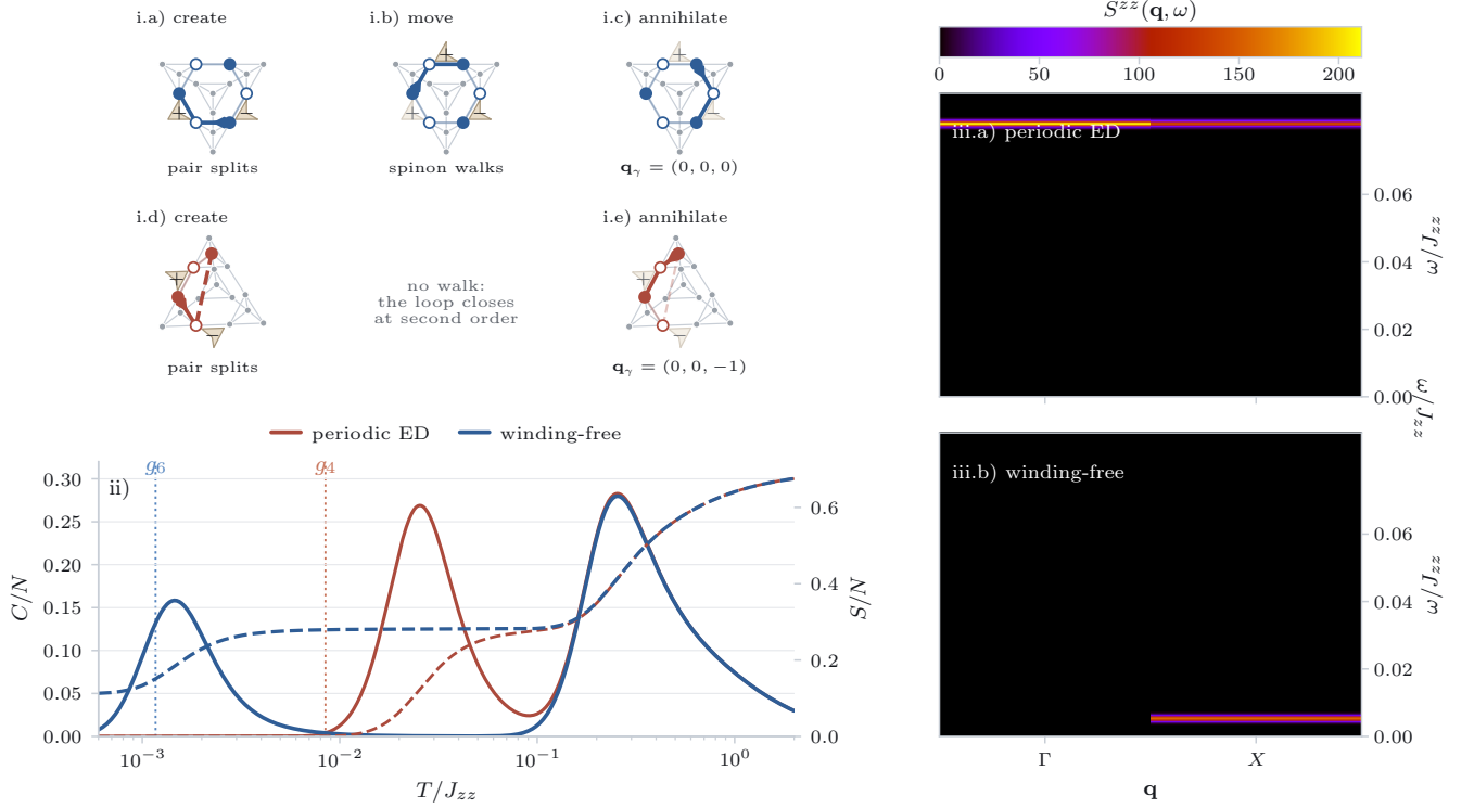
FIG. 1. Microscopic transport and winding removal on cubic-16. (i) One ring exchange, stage by stage, on the 16-site torus; gray dots and lines are the cluster and its intracell bonds, colored circles the loop, and filled versus open symbols the alternating S^z pattern the flip reverses. Each exchange flips both ends of one bond (highlighted, with the arrow); the tetrahedron it straddles stays neutral while the two outer ones change charge, so an exchange creates, moves, or annihilates a spinon–antispinon pair. A charged tetrahedron is shaded with its charge seated inside, and the pair left by the previous stage is faded. (i.a)–(i.c) The contractible hexagon: the first exchange splits a pair, the second walks the spinon on, and the third brings the two together and annihilates them. The sequence stays inside one cell and transports nothing, \mathbf{q}_\gamma = \mathbf{0} . (i.d),(i.e) The axial four-loop closes at second order, so it has no walking stage; its annihilating exchange is reached from the creating one only across a boundary-crossing bond (dashed). Lifted to the covering lattice the sequence is therefore an open path whose ends differ by \mathbf{q}_\gamma = (0, 0, -1) , and each charge annihilates against an image of its partner rather than the partner itself. The diagonal four-loop behaves identically with \mathbf{q}_\gamma = (1, 1, 0) . The source average of Eq. (10) keeps the hexagon and removes both four-loops. (ii) Heat capacity (solid, left axis) and entropy (dashed, right axis) at (J_\pm, J_{\pm\pm})/J_{zz} = (0.046, 0) , for ordinary periodic ED (orange) and the winding-free replacement of Eq. (11) at M = 4 (blue). Dotted vertical lines mark the perturbative scales g_6 and g_4 of Eqs. (2) and (3); the periodic low-temperature peak tracks the artifact scale g_4 , whereas the projected peak moves down to the ring-exchange scale g_6 . (iii.a),(iii.b) Zero-temperature longitudinal structure factor S^{zz}(\mathbf{k}, \omega) [Eq. (15)] for the periodic band h(\mathbf{0}) and the projected band h_{M=4} , on identical linear color scales. Both use the same canonically dressed microscopic S^z probe [Eq. (14)]; results are averaged over the three symmetry-related X points, with broadening \eta = 6 \times 10^{-4} J_{zz} .
