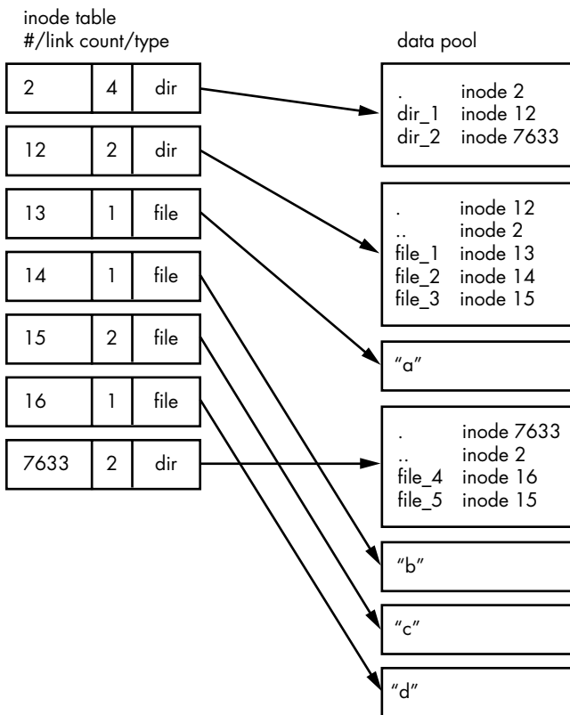
Figure 4-10: Inode structure of the filesystem shown in Figure 4-9
