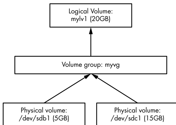
Figure 4-6: Results of reconfiguring logical volumes
