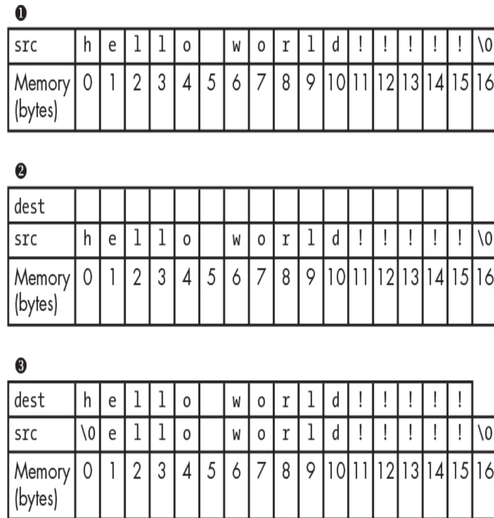
Figure 13-1: How memory overflows from dest to src
