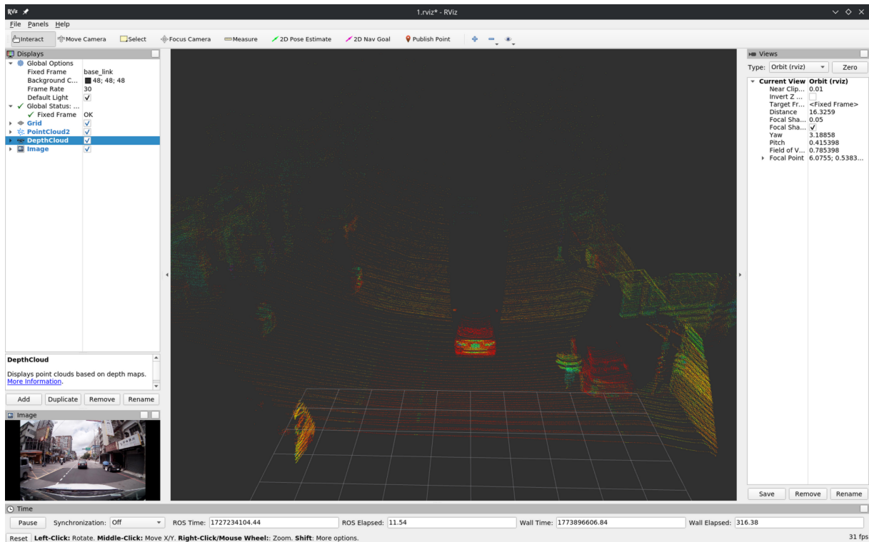
Figure 6: RViz pointcloud showcasing high-reflectivity objects alongside the camera image.
