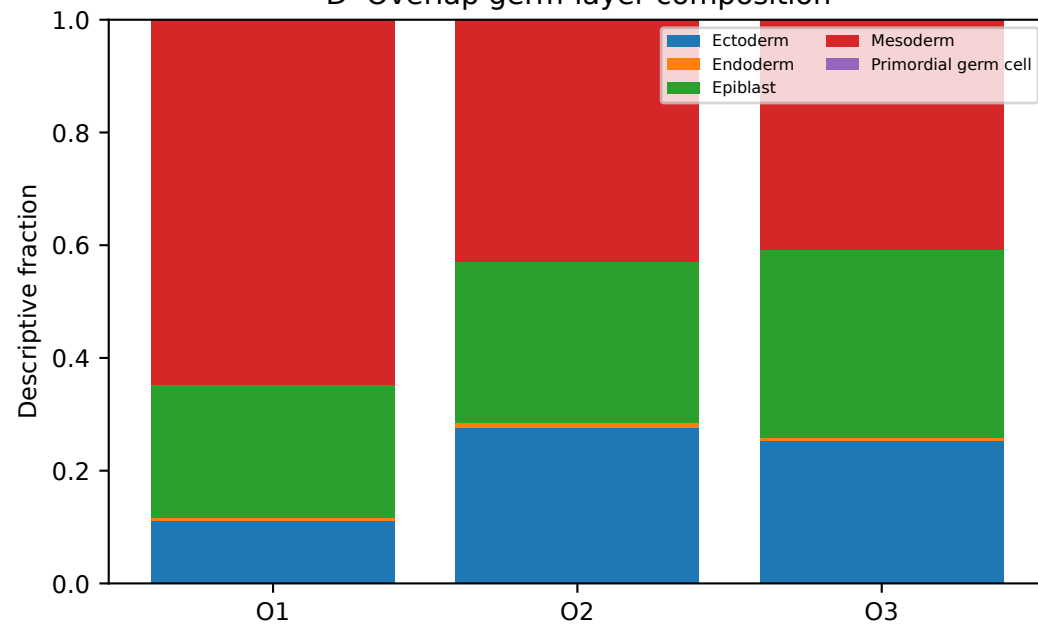
D Overlap germ-layer composition
