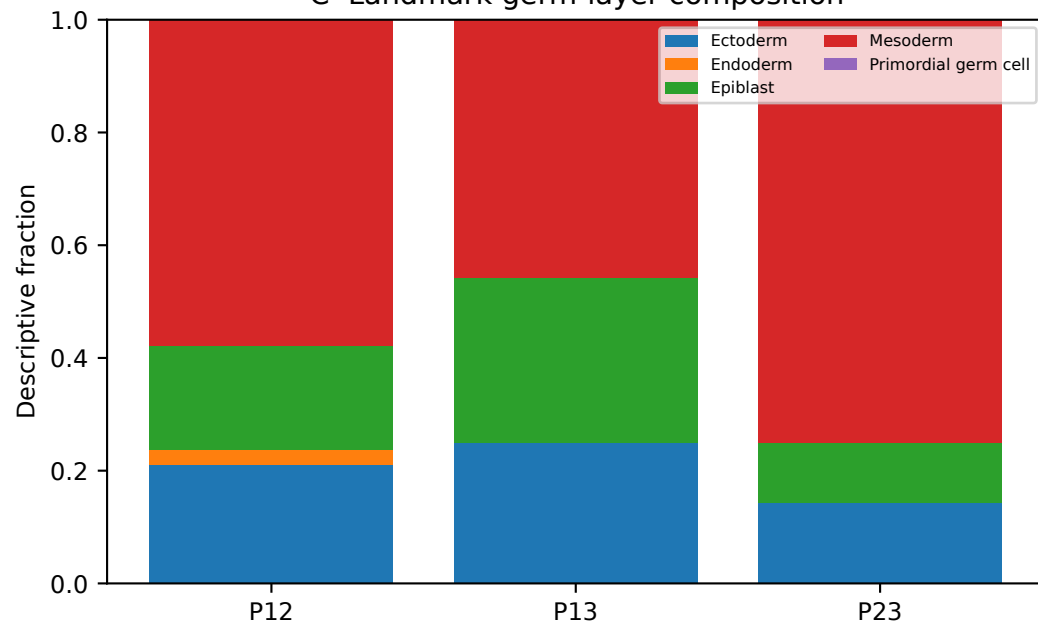
C Landmark germ-layer composition
