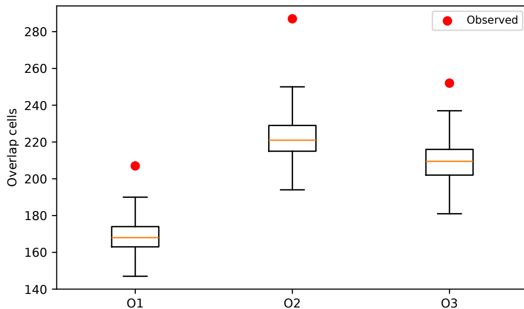
B Fixed-stratum S1 reference (B=1024)
