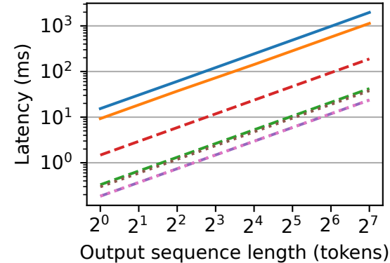
(c) GPT2 Decode Stage
