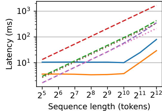
(a) BERT
