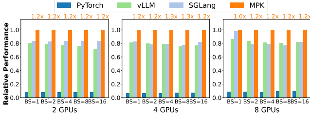
Figure 11: Multi-GPU comparison of MPK with existing systems for Qwen3-1.7B on H100 GPUs using tensor parallelism. All results are normalized to MPK; higher is better.
