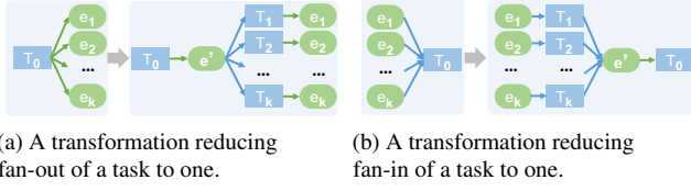
Figure 6: MPK performs graph transformations to normalize an arbitrary t Graph, ensuring that every task has at most one dependent event and at most one triggering event.
