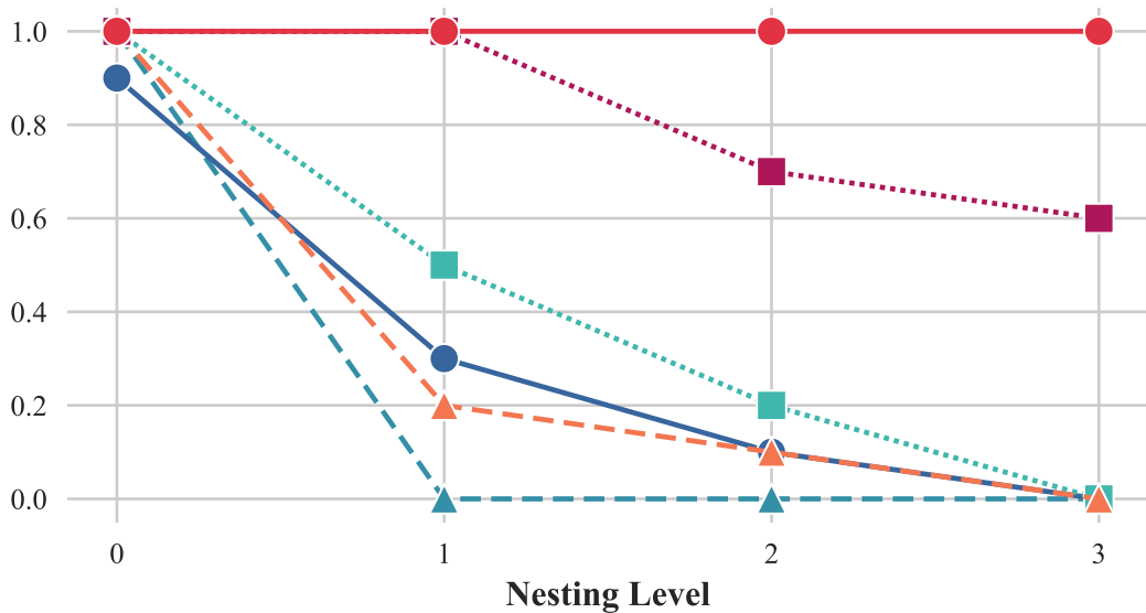
Accuracy
